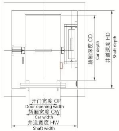
井道平面图 (担架梯) Shaft and car plan (Stretcher elevator)
