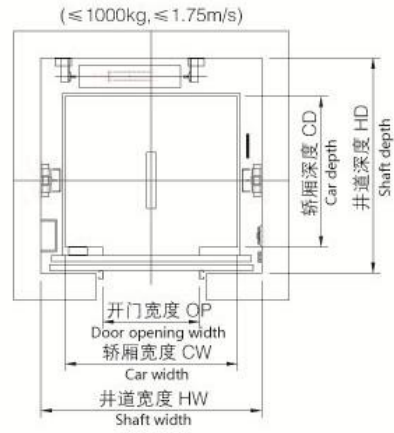
井道平面图 Shaft and car plan
