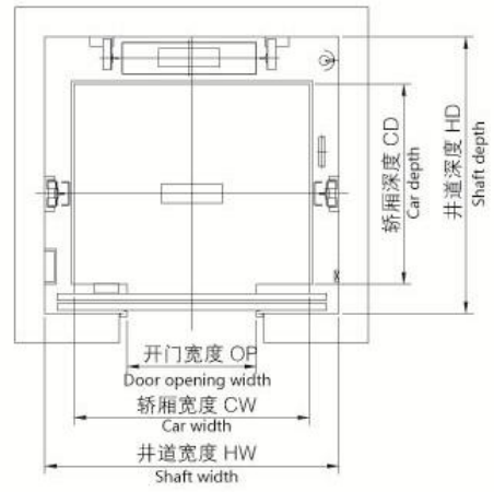
井道平面图 Shaft and car plan
