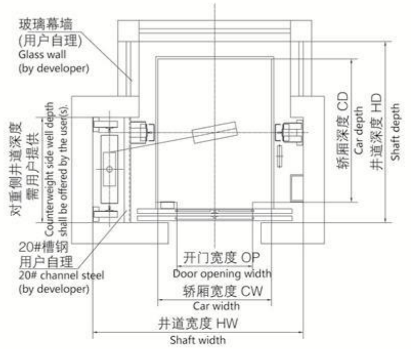
井道平面图 Shaft and car plan
